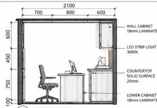
7 SECTION B-B SCALE 1:25
