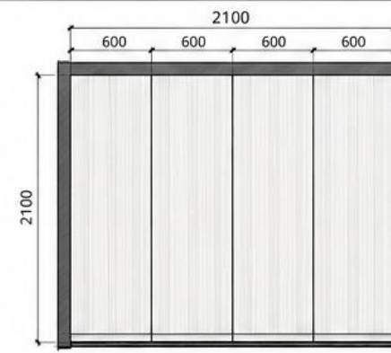
5 ELEVATION C (REAR WALL) SCALE 1:25
