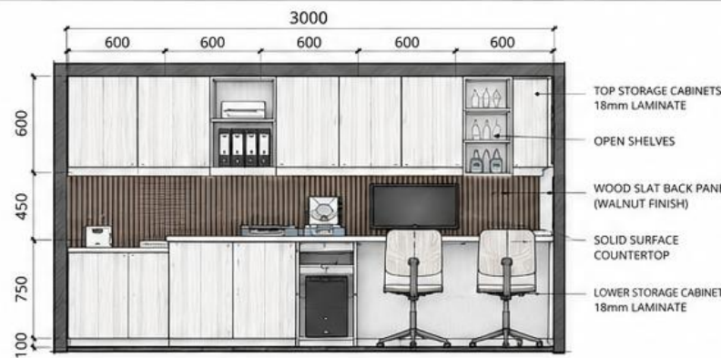
3 ELEVATION A (FRONT WALL WORKSTATION) SCALE 1:25
