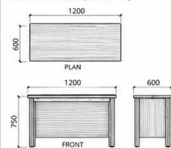
9 FURNITURE DETAIL (WORK DESK) SCALE 1:10
