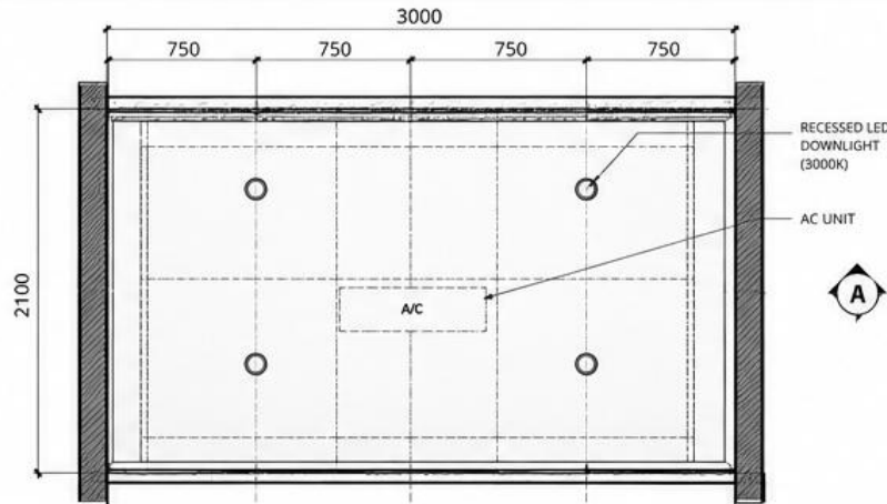
2 REFLECTED CEILING PLAN SCALE 1:25
